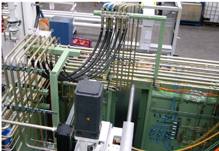
Fig. 11 Pipeline routing in a large machine
