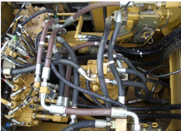
Fig. 32 Hose assemblies on a mobile hydraulic system
