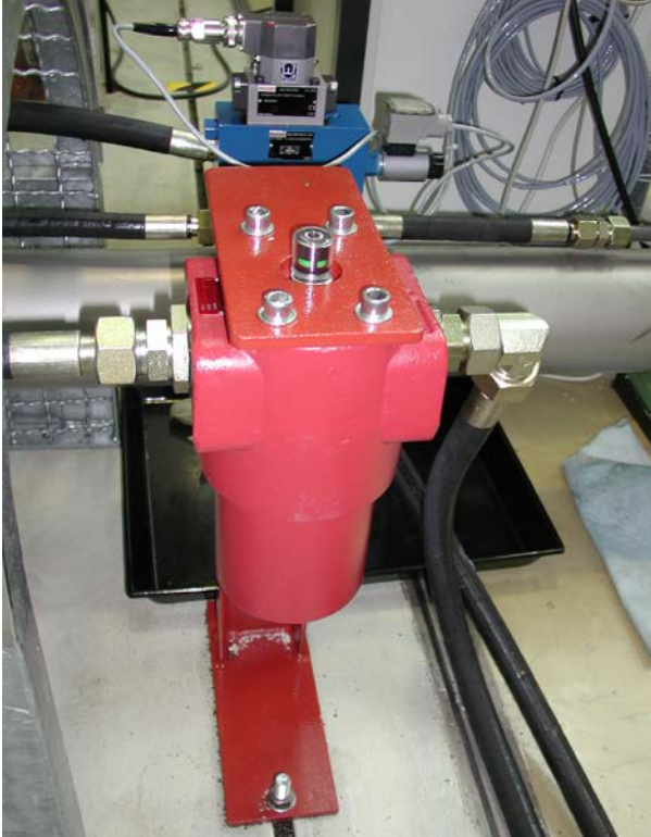
Fig. 23 Hydraulic filter with clogging indicator
