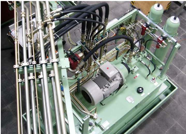
Fig. 9 Central hydraulic system at commissioning
