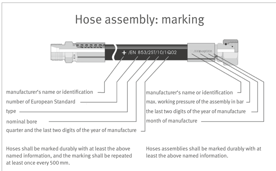
Fig. 13 Structure and labeling of a hose assembly
