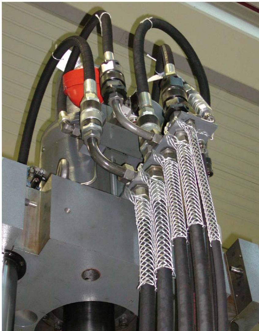
Fig. 17 Stripping protection on hose assemblies
