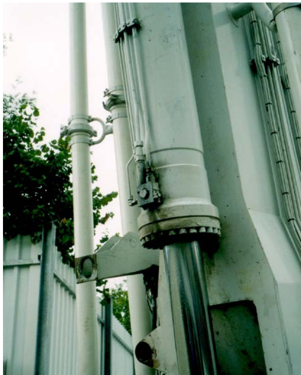
Fig. 18 Hydraulic cylinder with pilot-operated check valve
