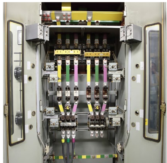
Fig. A 5-18 Opened panel
