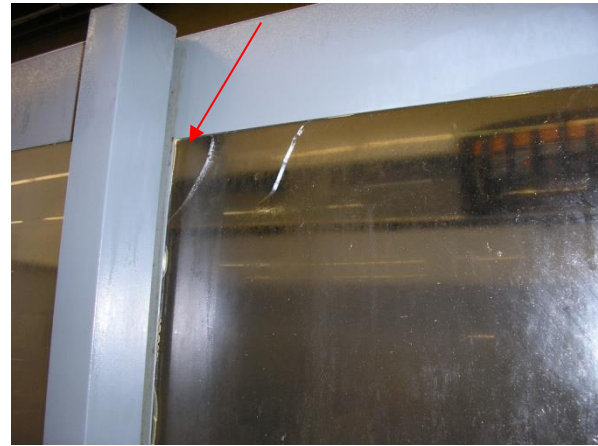
Cracks starting from the panel edge in embrittled polycarbonate panel
